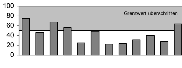
max. PM10-Tagesmittelwerte [µg/m 3 ]
